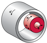
Internal cylindrical grinding
