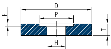
Grinding wheels 5
