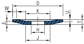
Grinding wheel 12 D / J x T / U x H - W x E x K
