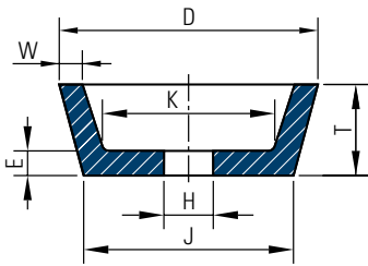
Grinding cup 11 D / J x T x H - W x E x K
