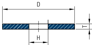
Grinding wheel 1 D x T x H
