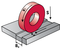
Profile grinding
