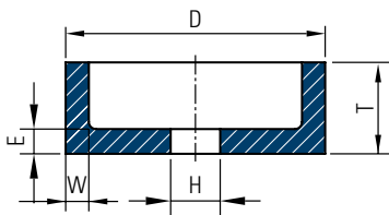
Grinding cup 6 D x T x H - W x E
