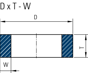
Grinding ring 2
