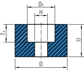
Grinding wheel 5 D x T x H - P x F
