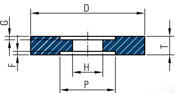
Grinding wheels 7
