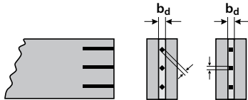
Dialette with MCD (monocrystalline diamond) pins:
