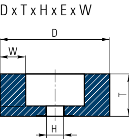
Grinding cup 6
