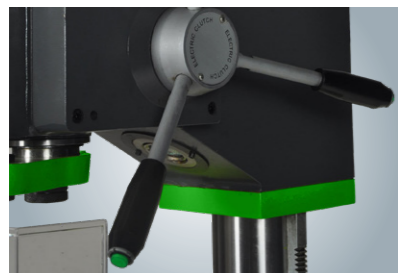
MK-4 electric clutch
